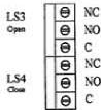
Extra Limit Switch (Dry Contact)
